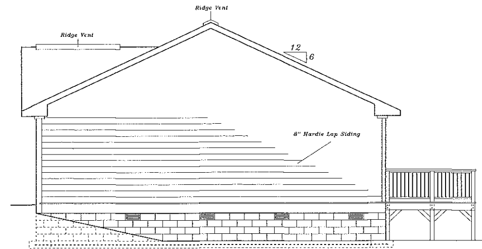
Right Side Elevations Scale : N/A
